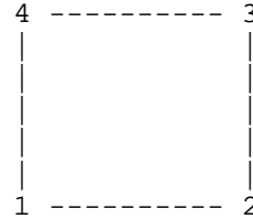
ESMF_MESHELEMENTTYPE_QUAD
