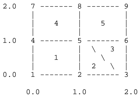
Node Id labels at corners Element Id labels in centers (Everything owned by PET 0)
