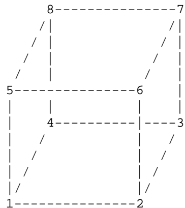
ESMF_MESHELEMENTTYPE_HEX
