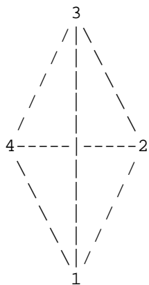
ESMF_MESHELEMENTTYPE_TETRA
