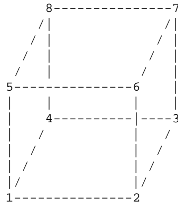
ESMF_MESHELEMENTTYPE_HEX
