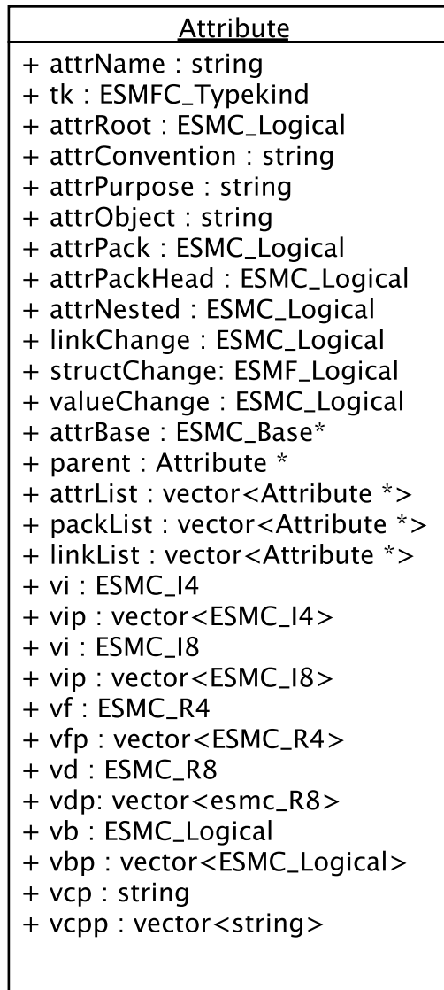
Figure 23: The structure of the Attribute class
