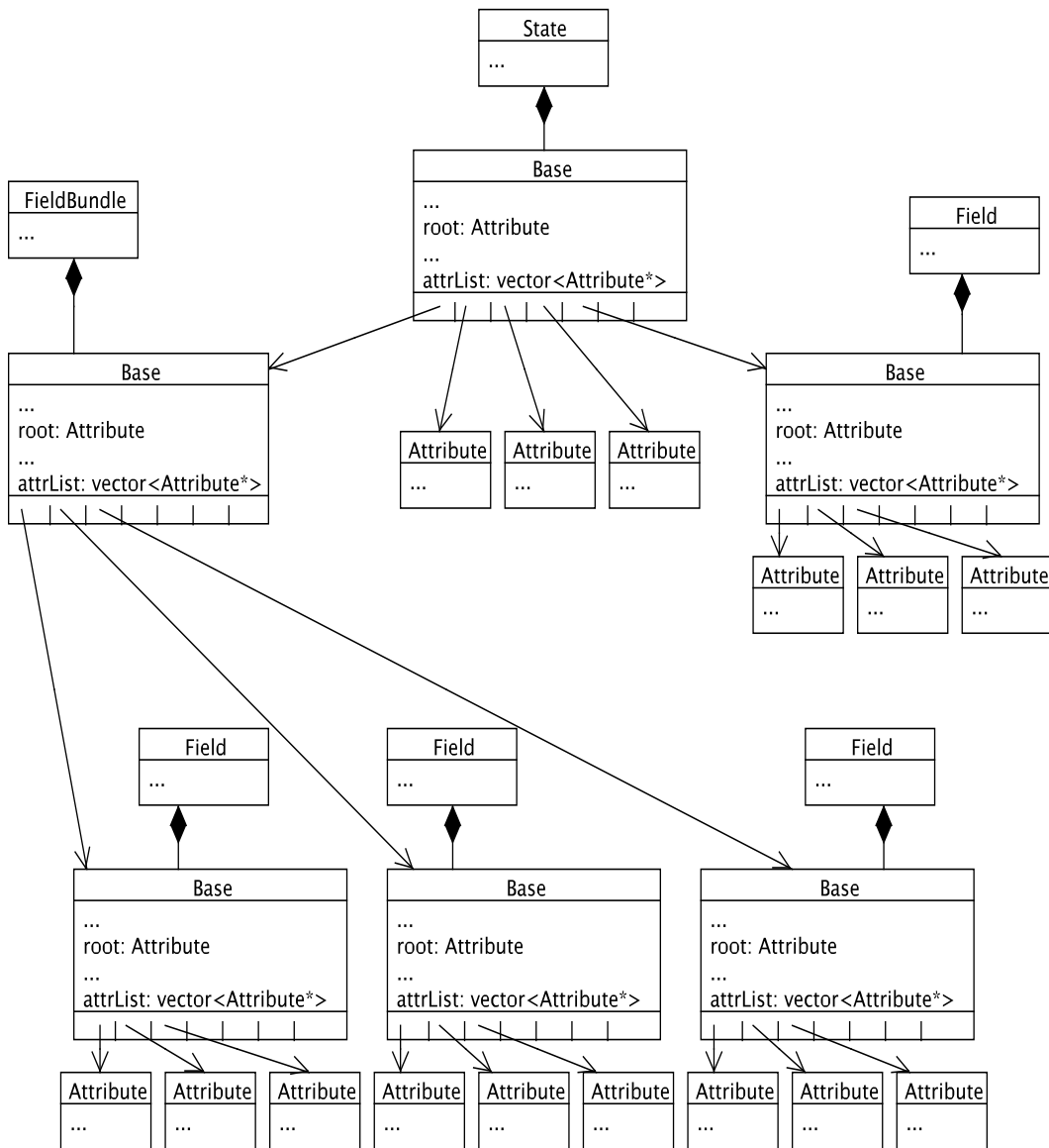
Figure 37: The internal object organization for the representation of Attribute hierarchies
