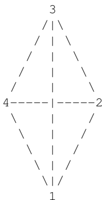
ESMF_MESHELEMENTTYPE_TETRA
