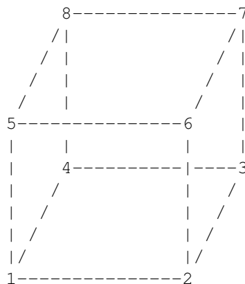
ESMF_MESHELEMENTTYPE_HEX
